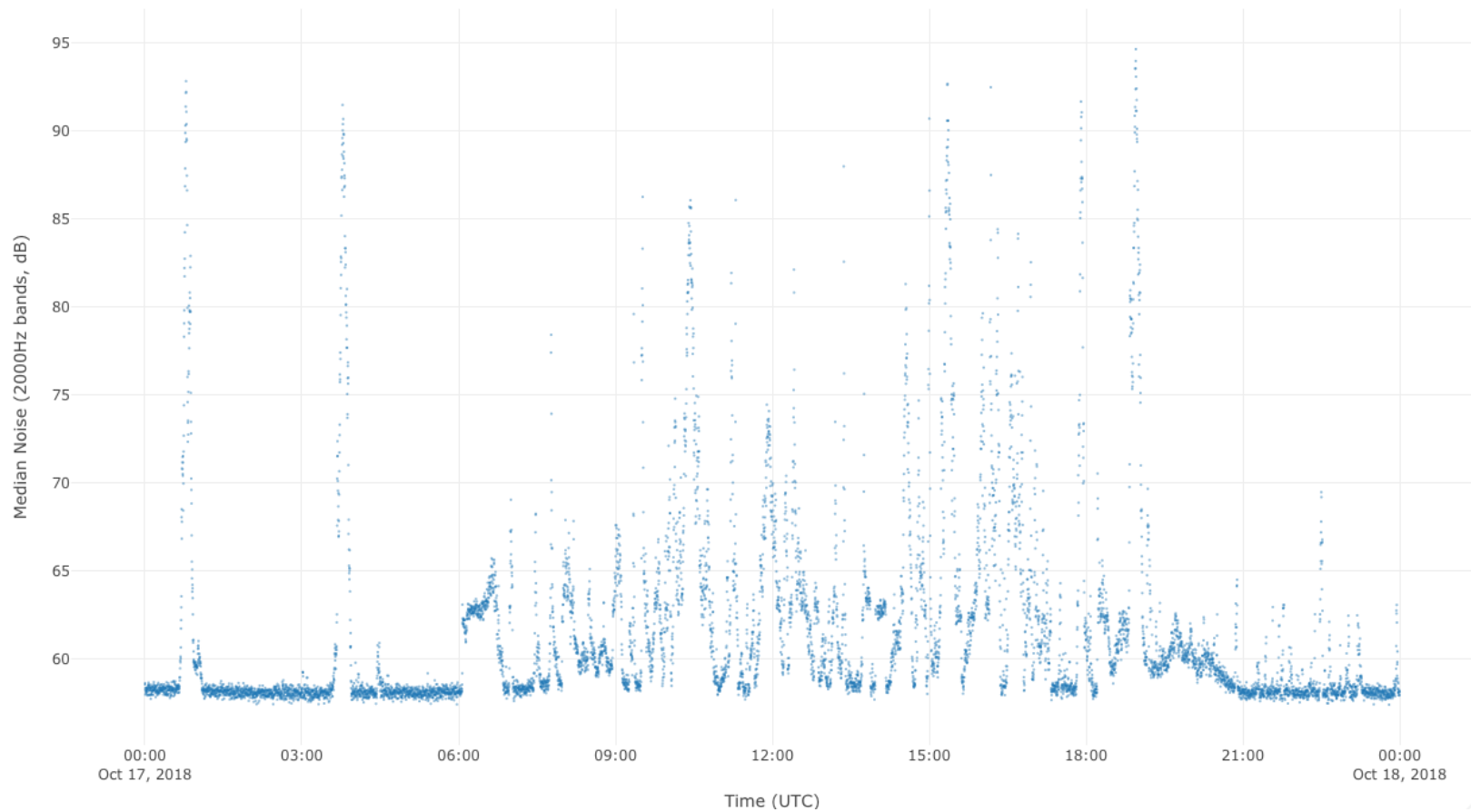
Noise Over Time for 17 October 2018
