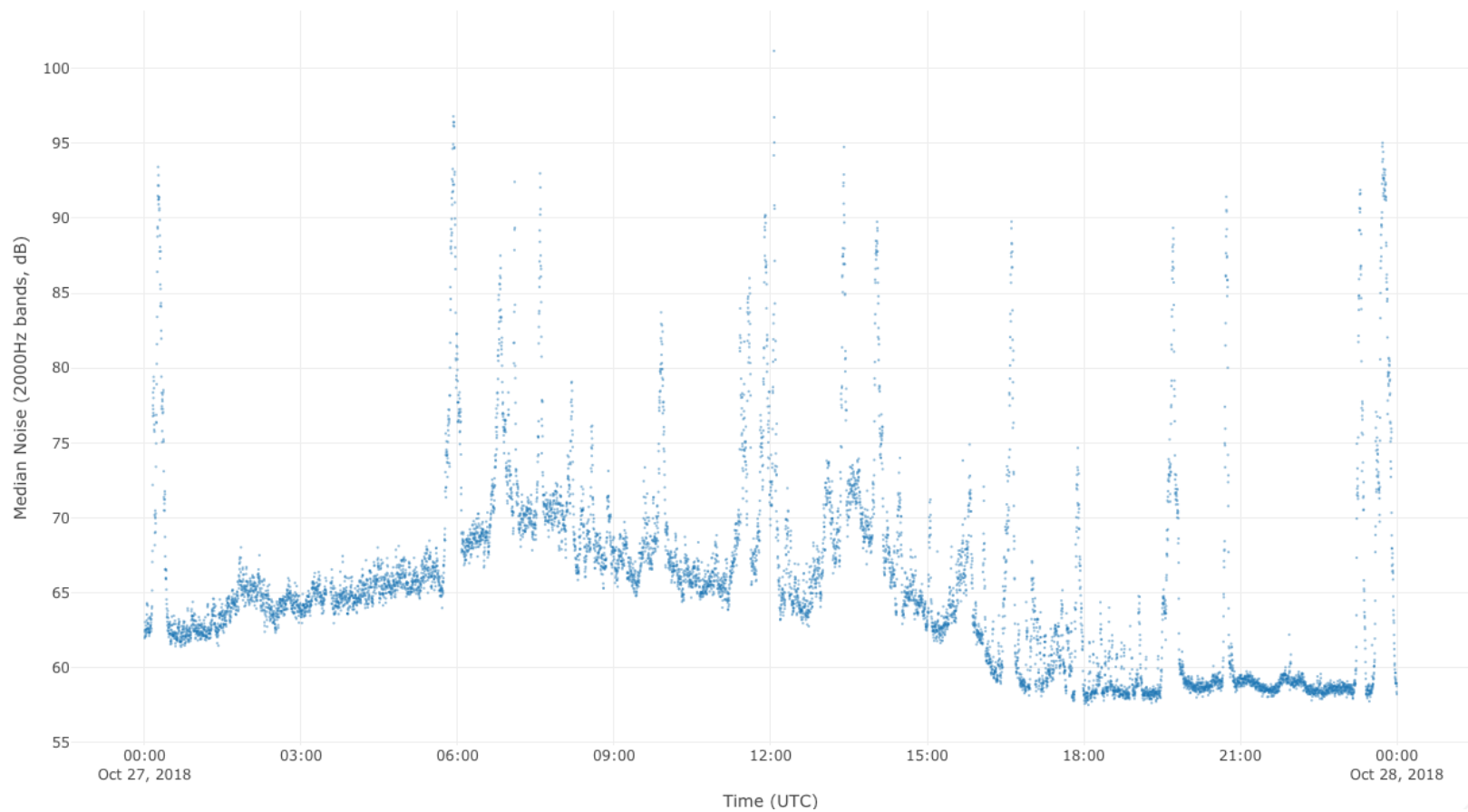
Noise Over Time for 27 October 2018
