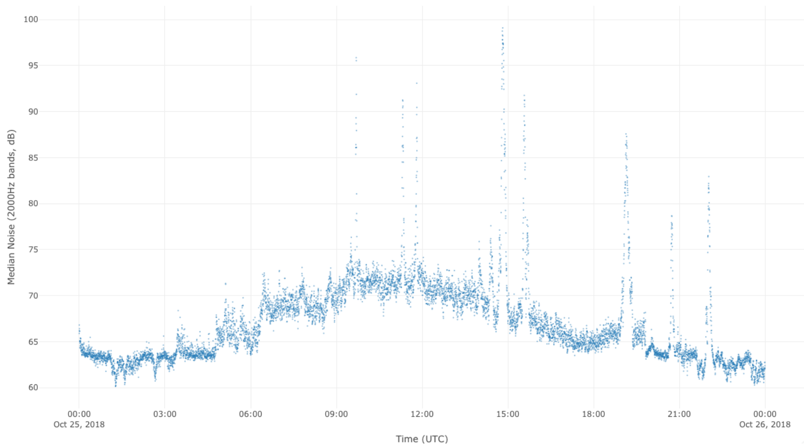
Noise Over Time for 25 October 2018
